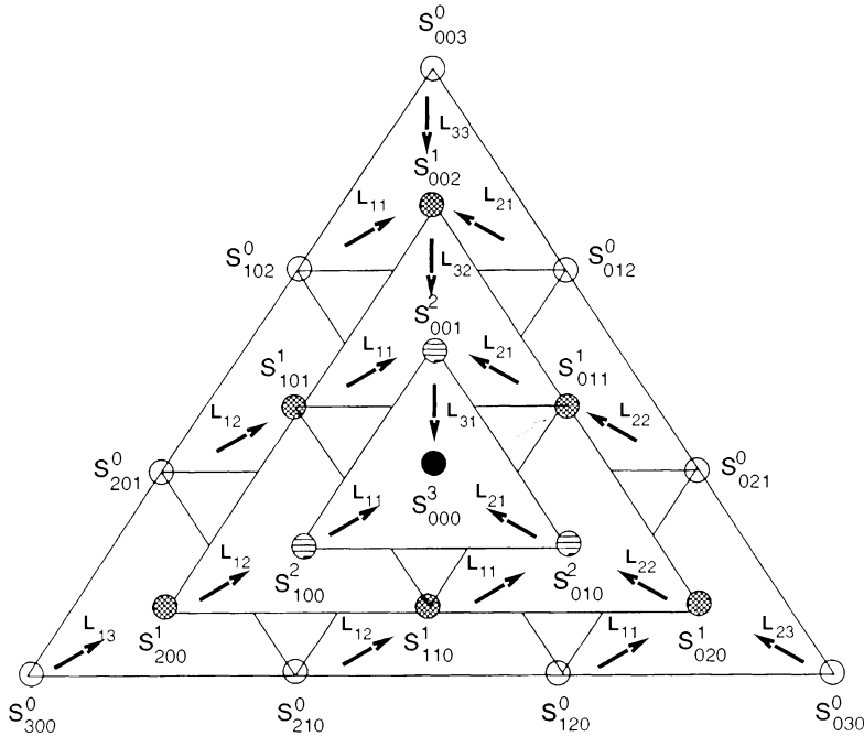
FIGURE 4. Nested multiplication evaluation algorithm for L-bases
